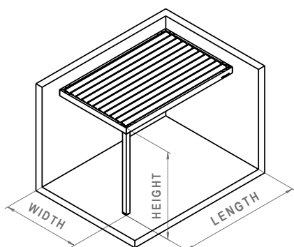
Type 5 - WALL-MOUNTED BLADES PARALLEL TO WALL
